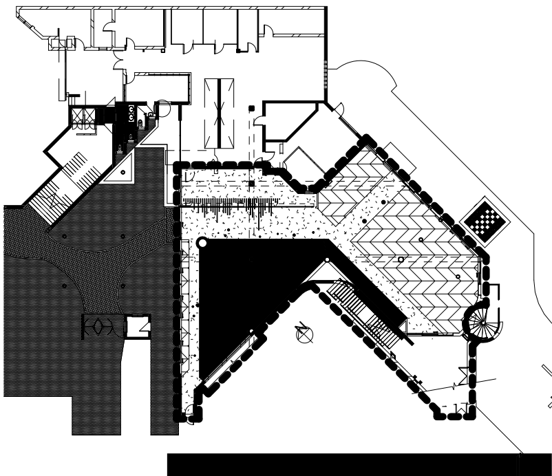
LOCALITY LAYOUT_Scale 1:500
